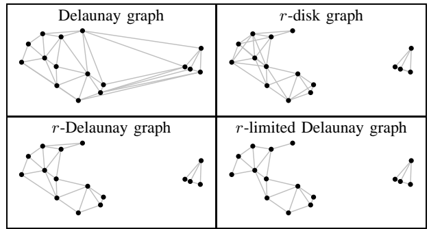
Fig. 1. Delaunay, r -disk, r -Delaunay, and r -limited Delaunay graphs for a random configuration of 16 generators with coordinates contained in the rectangle [0, 1.9] \times [0, .75] . The parameter r is taken equal to .45.
