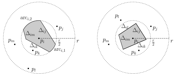
Fig. 2. The shaded regions are examples of sets V_i(\mathcal{P}) \cap B_{\frac{r}{2}}(p_i) . In the figure on the right, \partial V_i(\mathcal{P}) \cap B_{\frac{r}{2}}(p_i) does not contain any arc.
