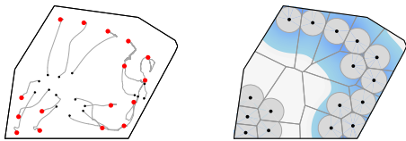
Fig. 4. Mixed centroid-area problem (with discontinuous agent performance f(x) = -x^2 \cdot 1_{[0, \frac{r}{2}]}(x) - \text{diam}(Q)^2 \cdot 1_{[\frac{r}{2}, +\infty)}(x) ): discrete-time algorithm T_{\text{ls}} for 16 agents on a convex polygonal environment. The left figure illustrates the gradient ascent flow and the right figure represents the final location and Voronoi partition. For each agent i , the intersection V_i \cap B_{\frac{r}{2}}(p_i) is plotted in light gray. After 13.5 seconds, the value of the multi-center function is approximately -6.803 .
