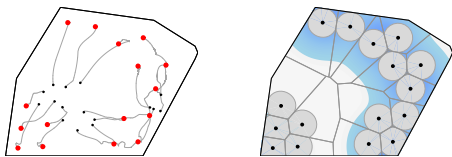
Fig. 3. Area problem (with agent performance f(x) = 1_{[0, \frac{r}{2}]}(x) ): discrete-time algorithm T_{\text{ls}} for 16 agents on a convex polygonal environment. The left figure illustrates the gradient ascent flow and the right figure represents the final location and Voronoi partition. For each agent i , the intersection V_i \cap B_{\frac{r}{2}}(p_i) is plotted in light gray. After 18 seconds, the value of the multi-center function is approximately 6.28977.
